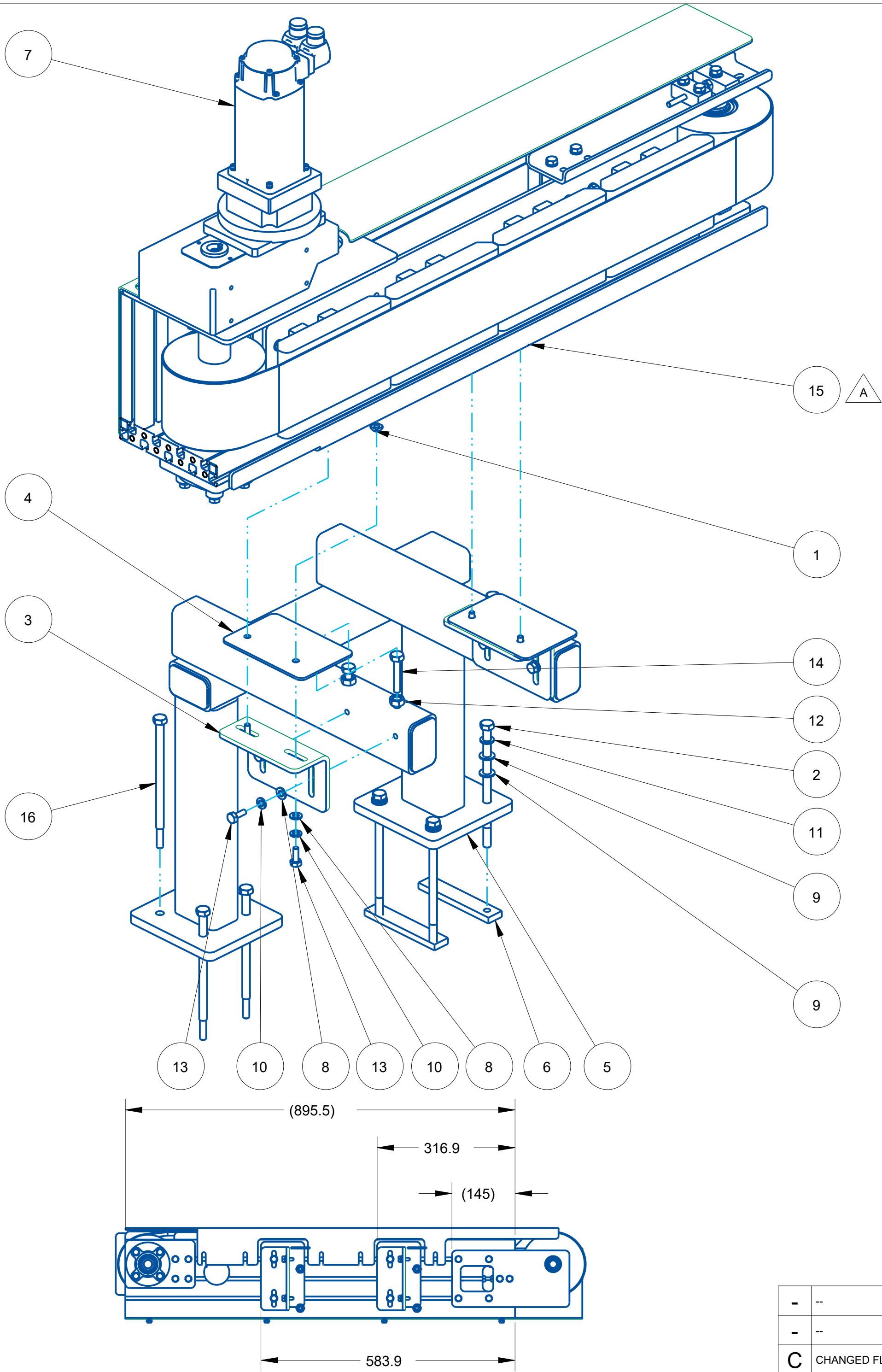
BOTTOM VIEW LEGS AND STRIPNUTS REMOVED FOR CLARITY SCALE 1/8
